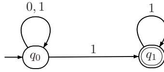
Figure 2.4: A nondeterministic Büchi automaton recognizing the \omega -language L = (0 \cup 1)^*1^\omega .
